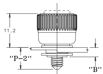
FASTENED PART NUMBER: 47-80-3X1-Y0 SHOWN
