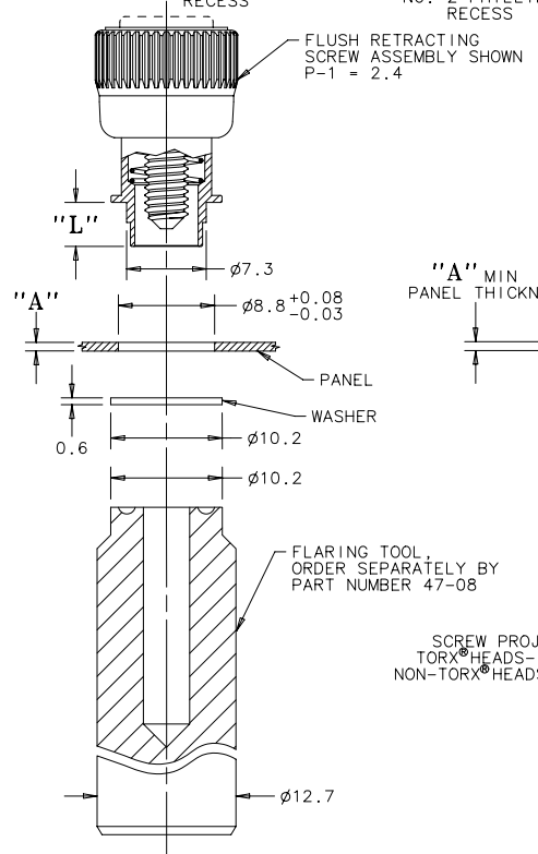
PANEL PREPARATION PART NUMBER: 47-80-3X1-Y0 SHOWN
